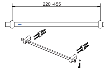
Recommended center distance 220~455mm ACC2413 Single Towel Rail 500mm
