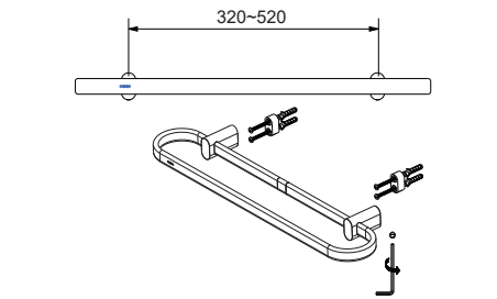
Recommended center distance 320~520mm ACC2402 Double Towel Rail 650mm
