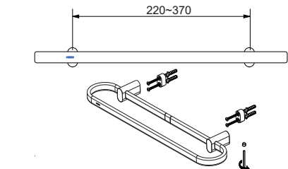
Recommended center distance 220~370mm ACC2412 Double Towel Rail 500mm
