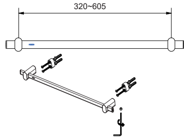
Recommended center distance 320~605mm ACC2403 Single Towel Rail 650mm
