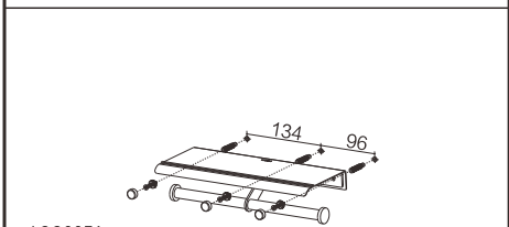
ACC9971 Double Paper Holder Wlid
