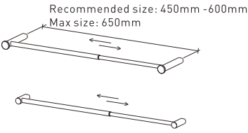
ACC9974 Bath Towel Bar
