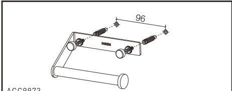
ACC9973 Paper Holder
