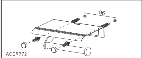
ACC9972 Paper Holder Wlid
