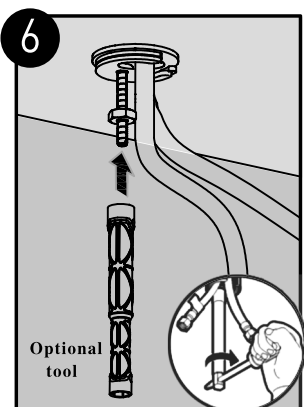
用扳手或选配工具锁紧螺母 Use wrench or optional tool to tighten the nut
