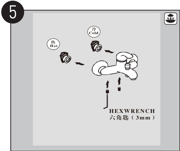
特殊之字接头产品。 请注意密封O型圈的使用。 Product with general inlet elbow. Please check the o-ring in the two inlet elbow.
