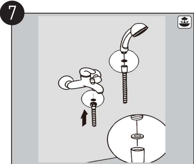
请注意密封垫圈的使用 Please check the washer between faucet and elbow.
