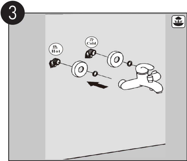
普通之字接头产品。 请注意密封垫圈的使用。 Product with general inlet elbow. Please check the washer between faucet and elbow.
