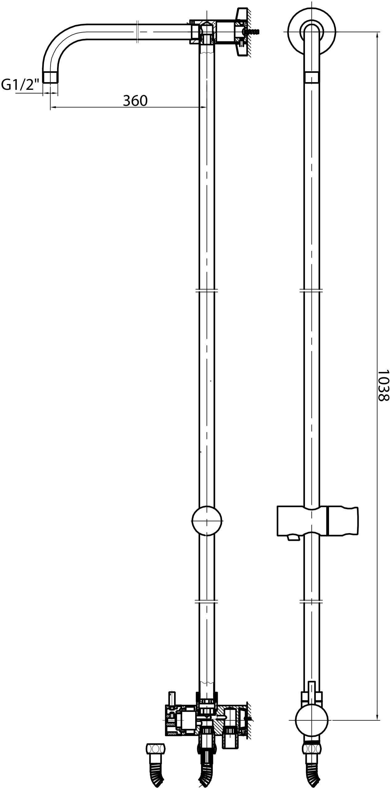
SKU: 2232 Shower Bar with diverter & bracket (Shower hose connection)
