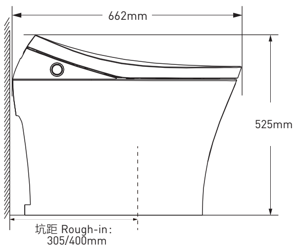
侧面图 Side View
